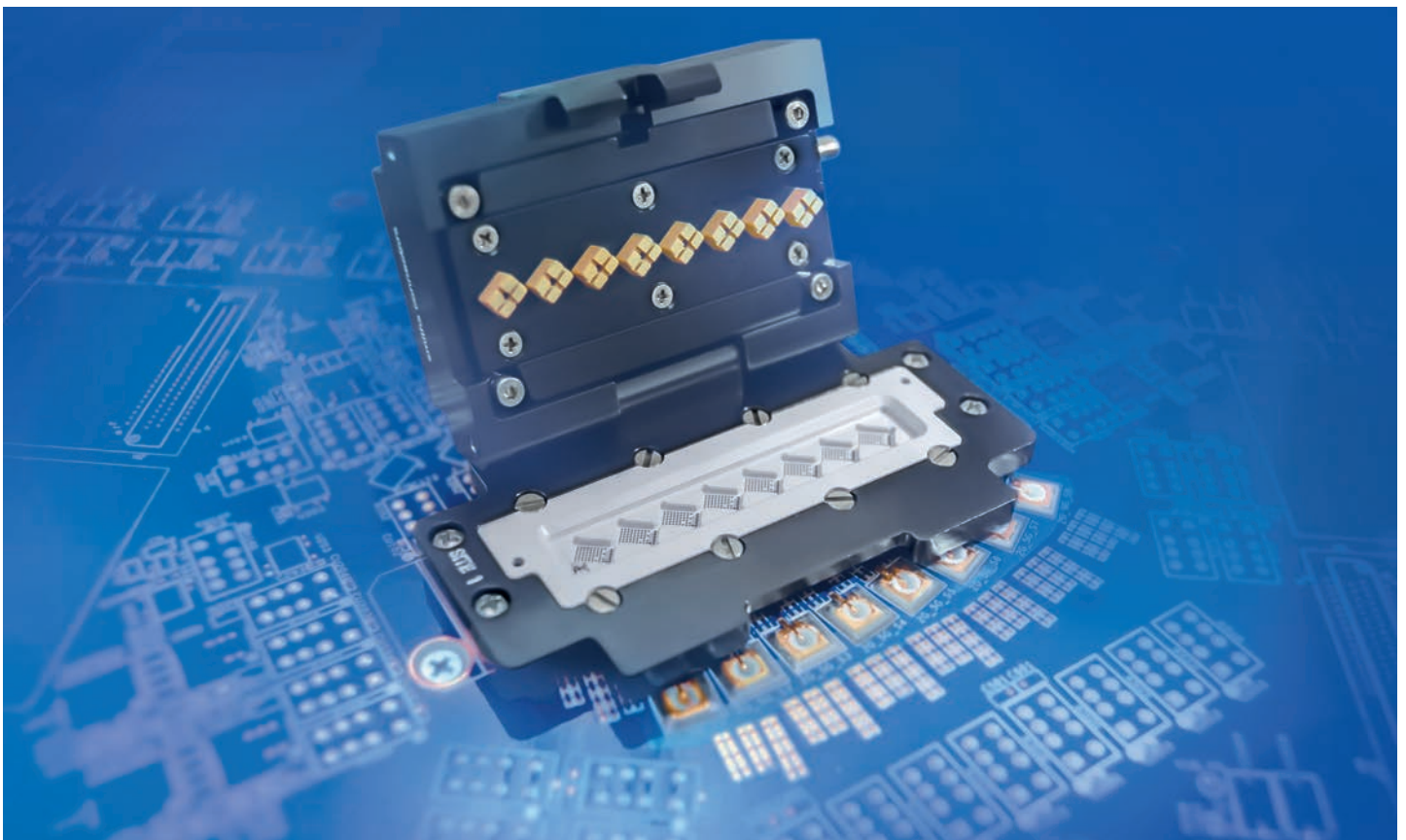
Manual Actuator for Sorted Die Test
