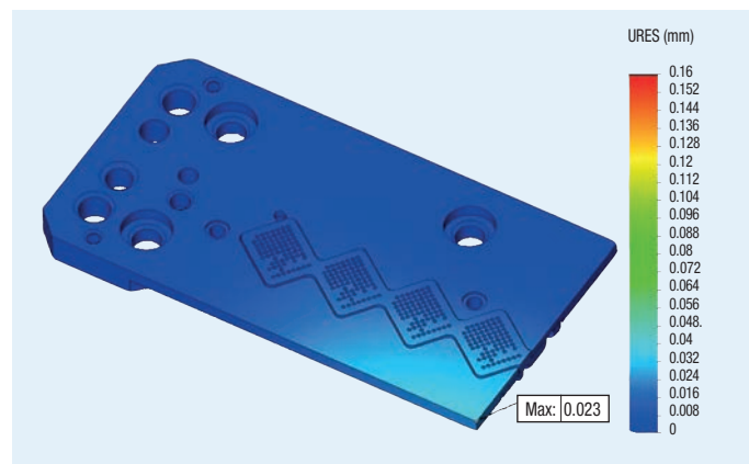
SST Frame & Proprietary Material "PEEK Rigid" Body
