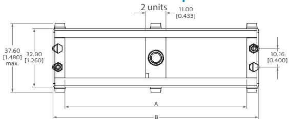
LEMVL Receptacle
