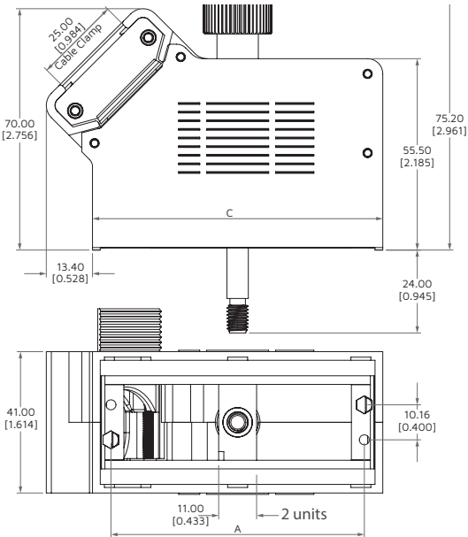
LEMVL Receptacle
