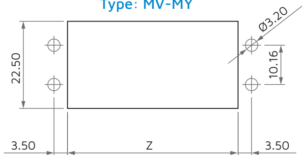
Type: MV-MY
