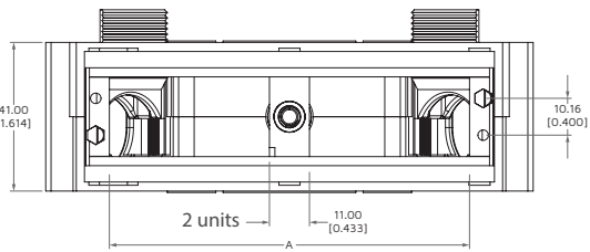
LEMVL Receptacle
