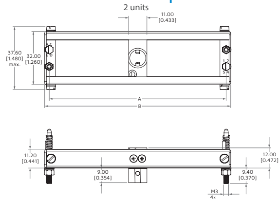
LEMY Receptacle
