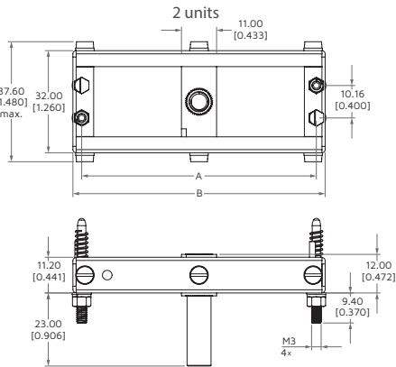
LEMVL Receptacle
