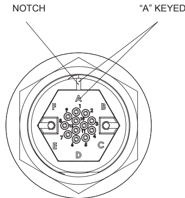
KEYING POSITION A Receptacle Wiring End
