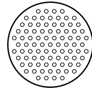
85x SPRING PROBE CONTACTS (Custom Mating Face)
