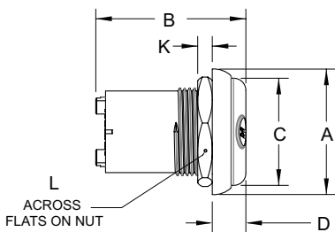
[E] RECEPTACLE
