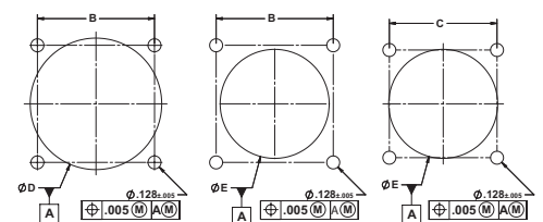
BACK PANEL MOUNTING
